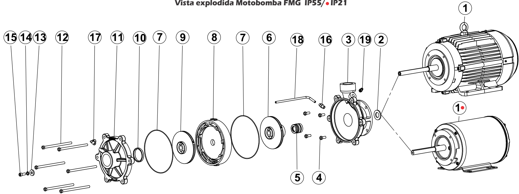
Vista explodida Motobomba FMG IP55/•IP21
