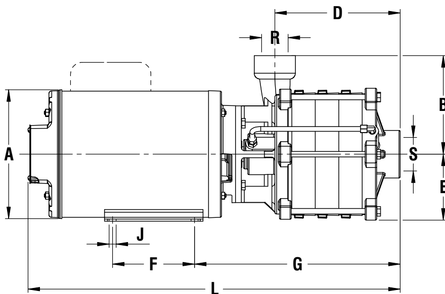
Dimensional Motobomba FMG IP21 •
