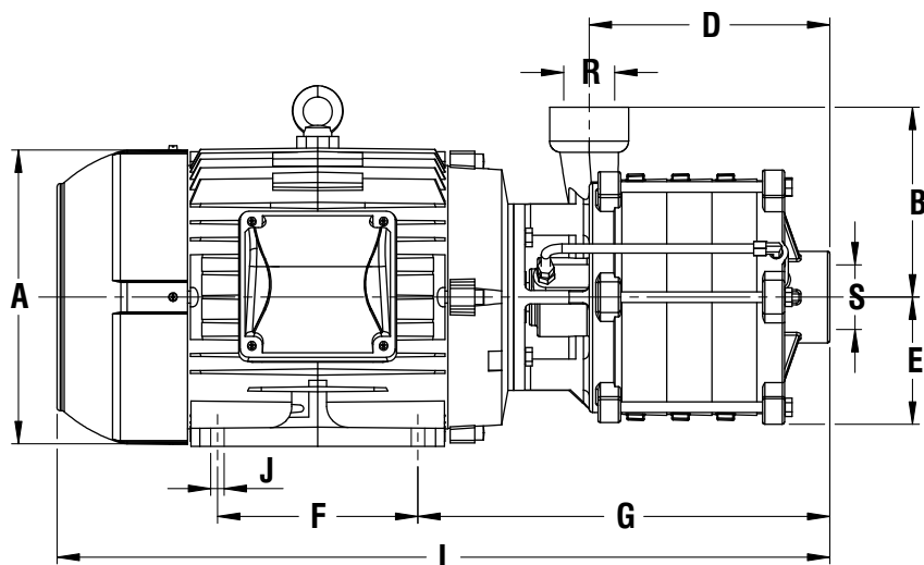
Dimensional Motobomba FMG IP55
